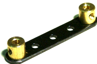
Double crank, 3 round holes, 2x brass boss M4
